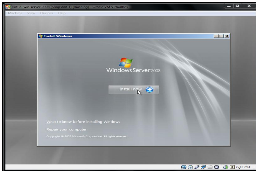
Gambar 7. 6 : Instalasi Winserver 2008
