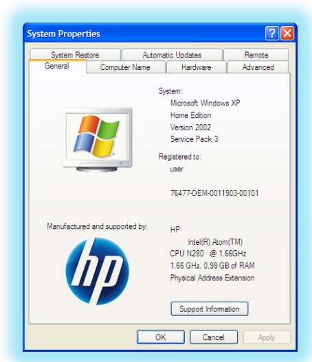
Gambar 4.1 System Properties
